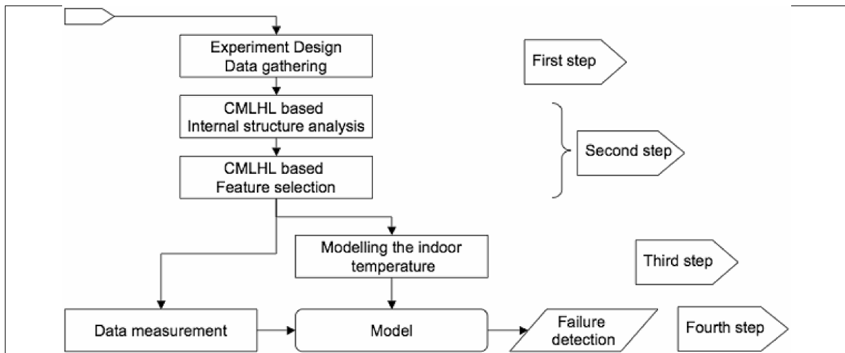
Fig. 3. The schema of the IKBIS to detect thermal insulation failures. The relevance of CMLHL is apparent in two ways as it allows the relevant features to be selected i.e., to reduce the variables used to train and to analyse the internal structure of the data set.
