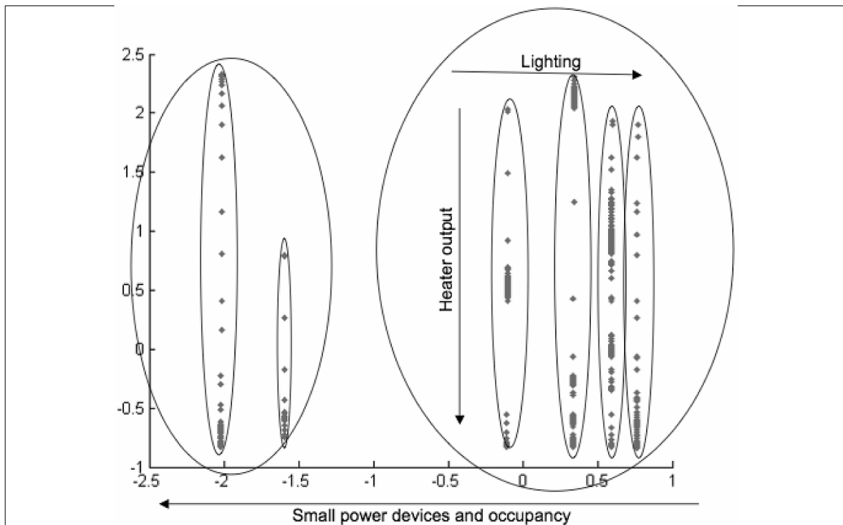
Fig. 5. The CMLHL projection. As can be seen, there are four relevant features that allow the indoor temperature to be modelled: the occupancy, the small power devices total power, the lighting electrical power and the heating system power.
