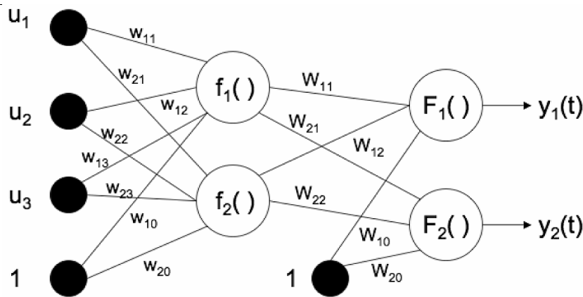
Fig. 2. A MLP network with two layers, with two nodes per layer, and three inputs. W_{ij} is the weight matrix between the hidden and output layer, while w_{ij} is the weight matrix between the inputs and the hidden layer. The network has two bias nodes with value 1.
