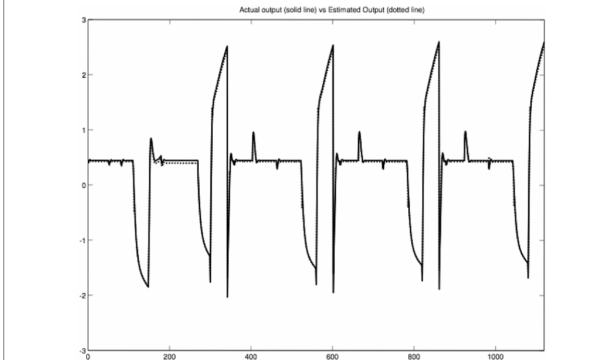
Fig. 9. Case of study: the city of Ávila. Output response of NNARX model for the validation data set. The actual output (solid line) is graphically presented with one-step-ahead prediction (dotted line). The X-axis represents the time steps, the Y-axis represents the signal value.
