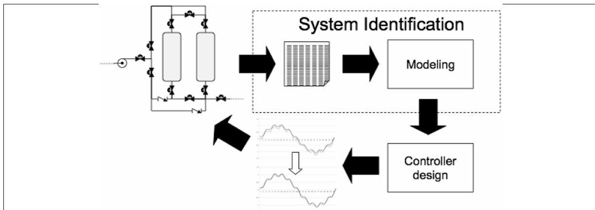
Fig. 1. The data source cycle: the data is gathered through the sensors from a process in operation – the set of valves and the tanks in the figure. This data is then processed and a better controller is found. The controller is then used. Whenever the behaviour of the system may be improved the cycle is repeated.
